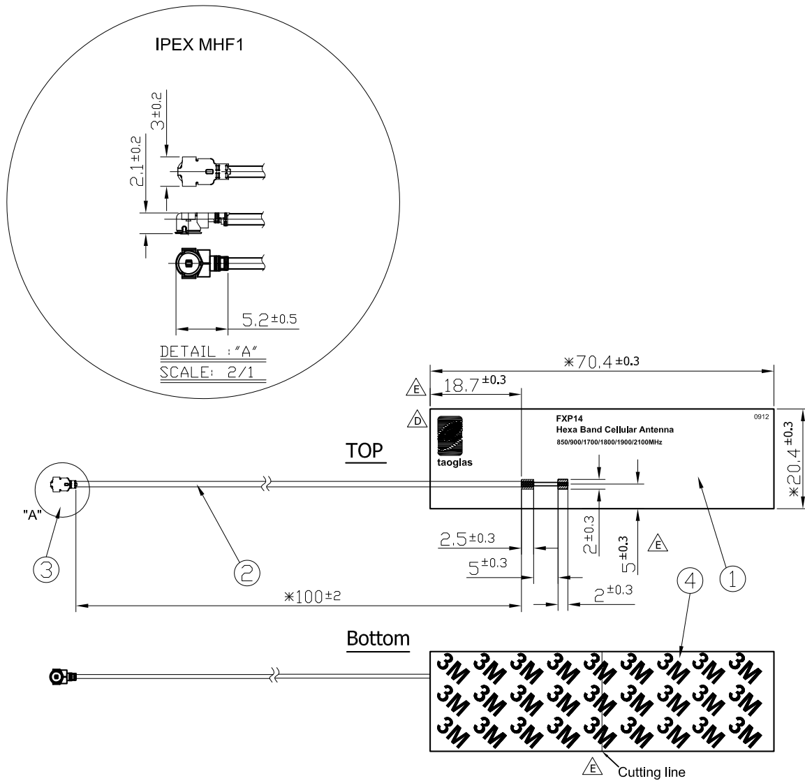
Figure 10. Mechanical Drawing for the FXP14 Antenna
